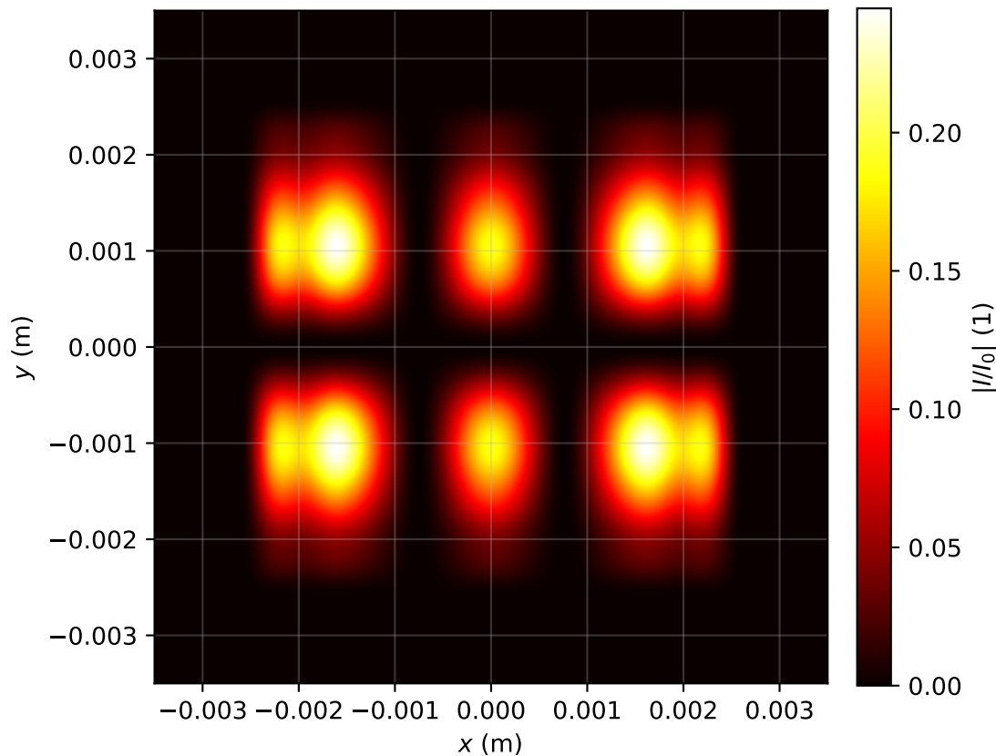
Intensity profile I(x, y, z = 3.742)/I_0 , P_{in}=0.5P_{cr} , artificial time
